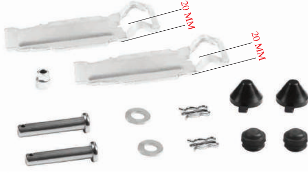
111K114 İPAT TUTUCU TAMİR TK. BRAKE PAD RETAINER KIT
