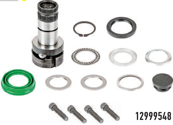
279K103 > KALİPER ŞAFT TAKIMI / CALIPER SHAFT SET -R
