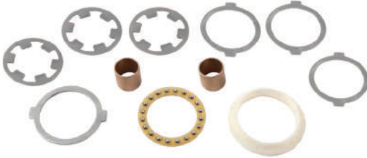
302K103 > KALİPER MEKANİZMASI TAMİR TAKIMI MECHANISM REPAIR KIT
