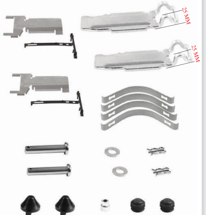
111K113 İPAT TUTUCU TAMİR TK. BRAKE PAD RETAINER KIT
