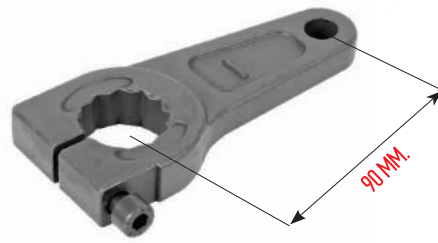
314K103 > KALİPER ŞAFT LEVYESİ CALIPER SHAFT LEVER
